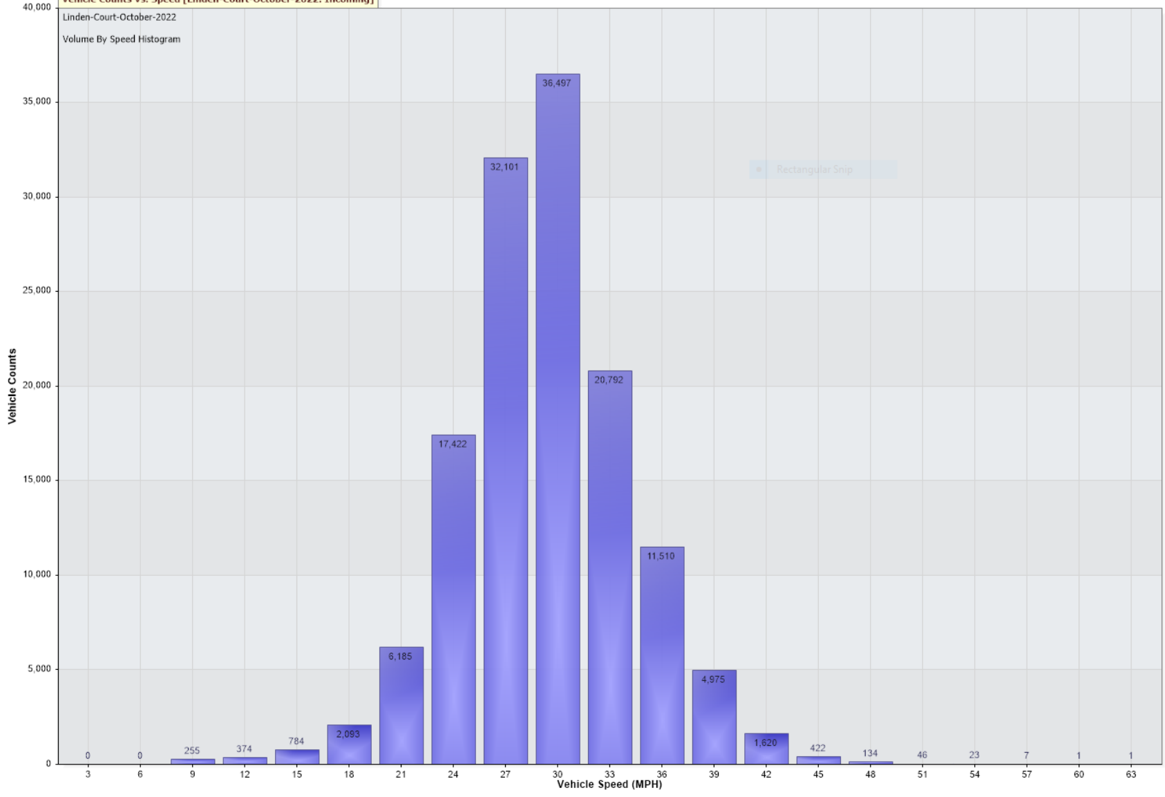
Vehicle Counts Vs. Speed [Linden-Court-October-2022: Incoming]
