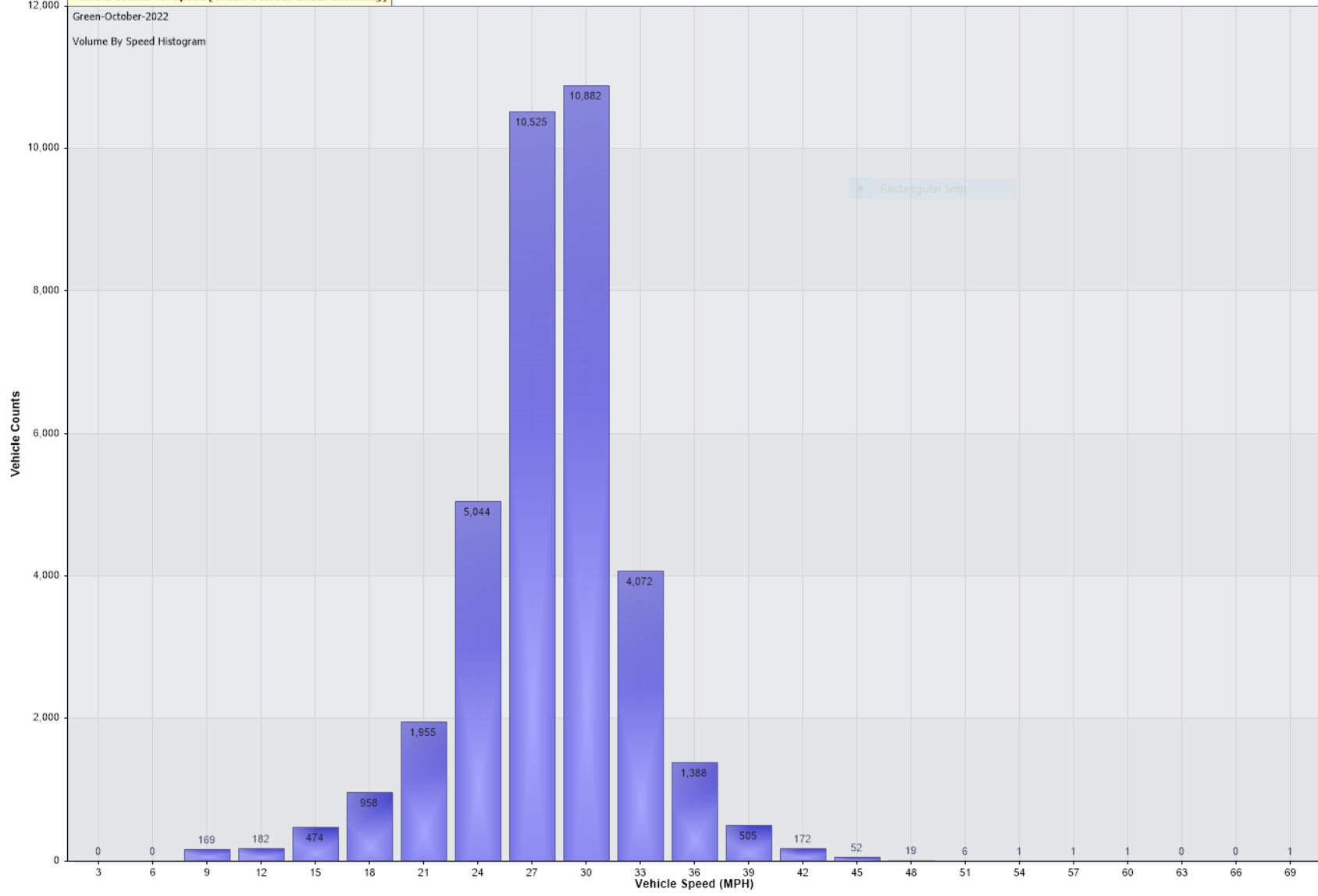
Vehicle Counts Vs. Speed [Green-October-2022: Incoming]
