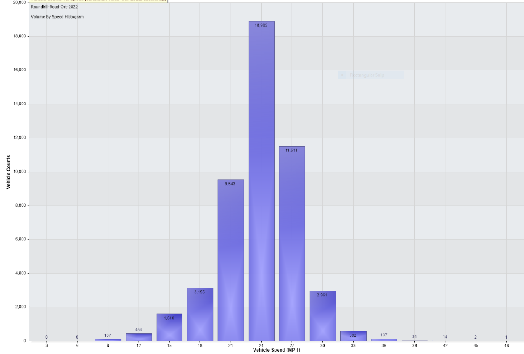
Vehicle Counts Vs. Speed [Roundhill-Road-Oct-2022: Incoming]
