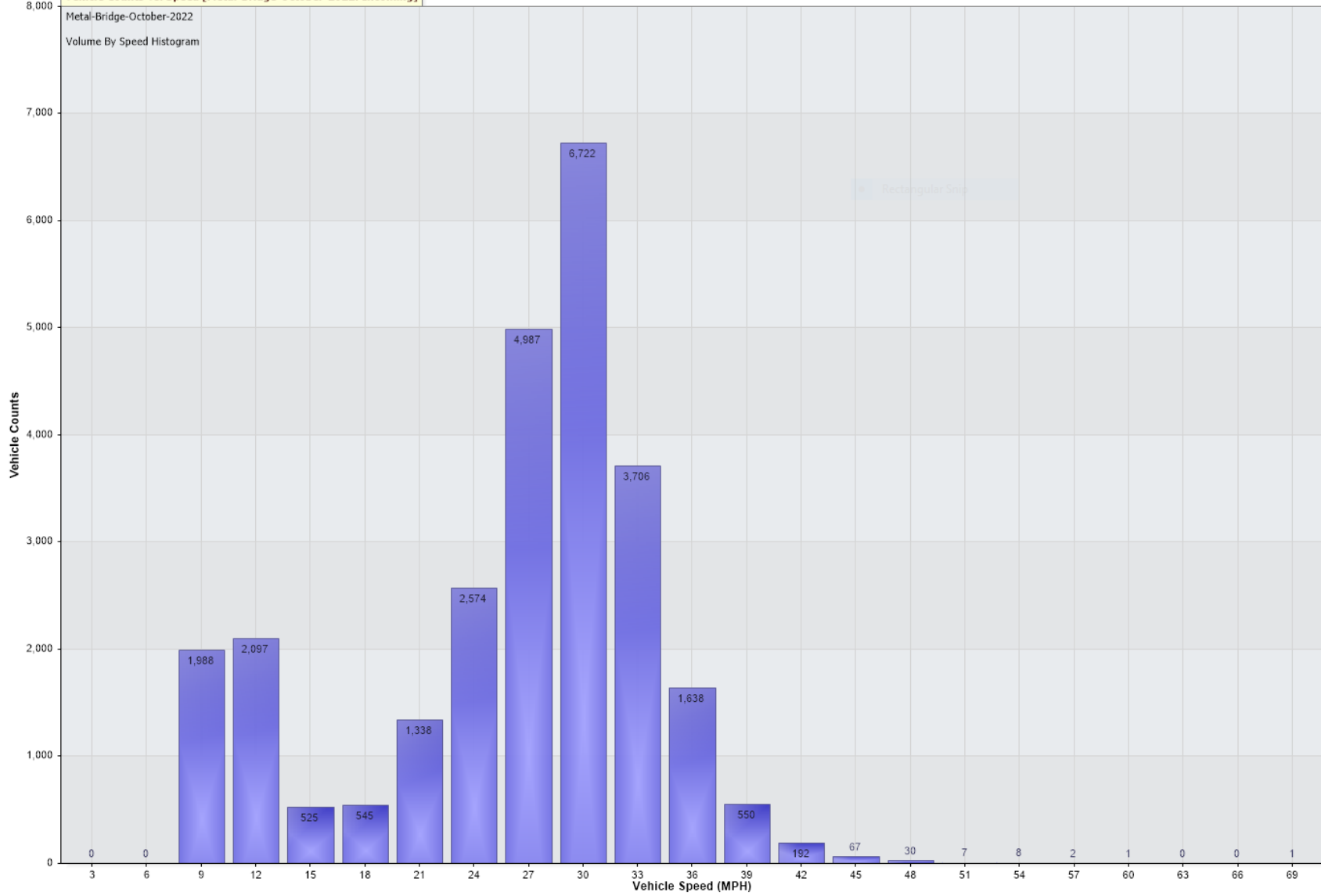
Vehicle Counts Vs. Speed [Metal-Bridge-October-2022: Incoming]
