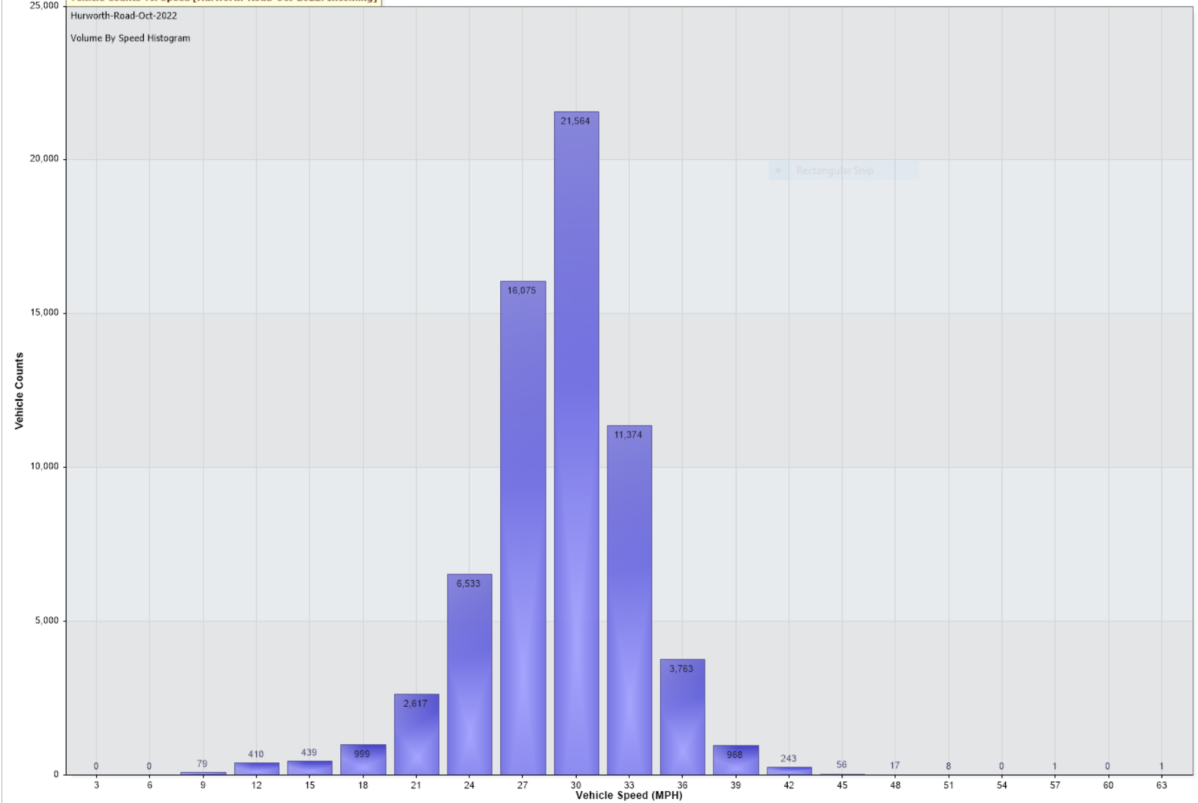
Vehicle Counts Vs. Speed [Hurworth-Road-Oct-2022: Incoming]
