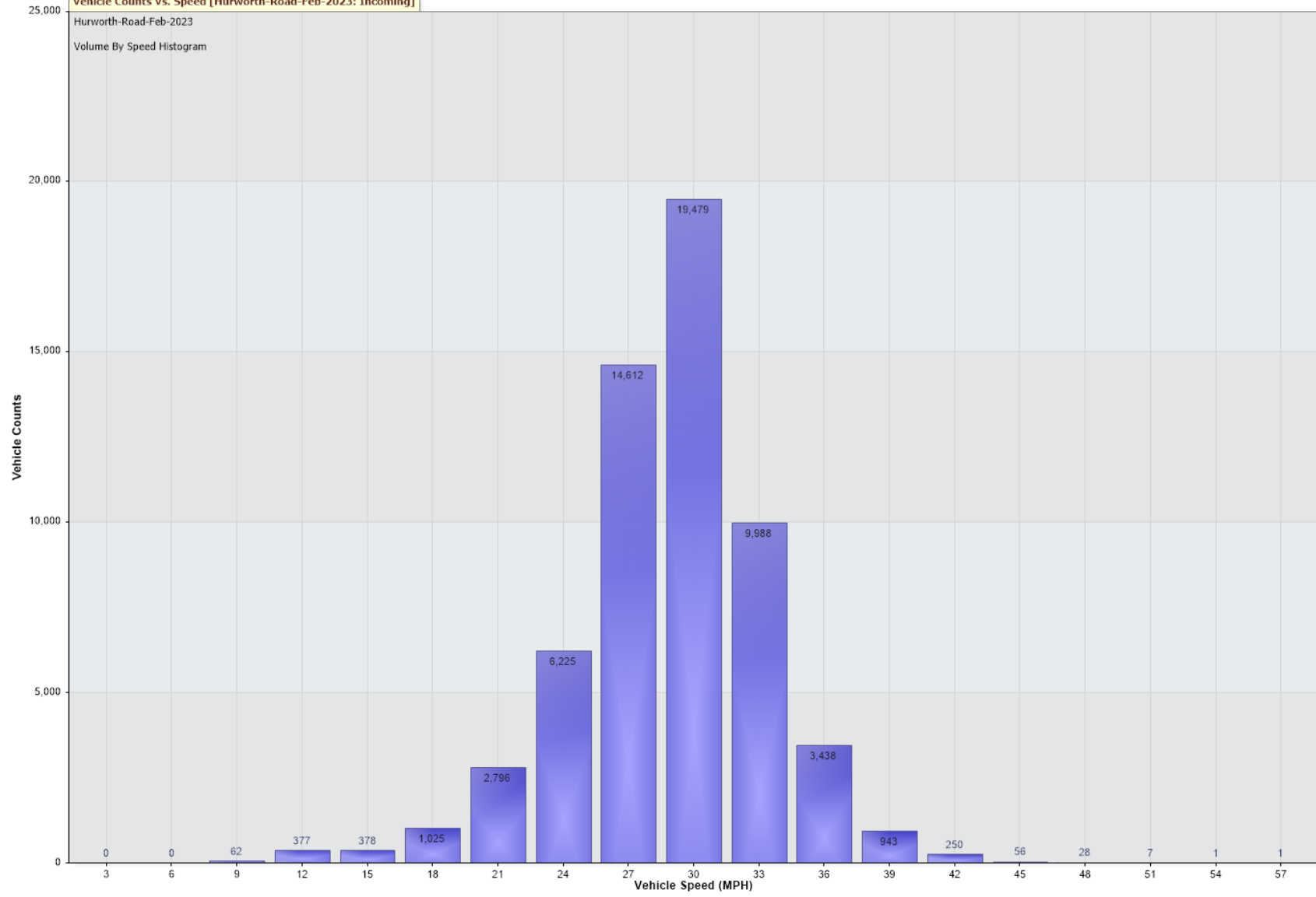
Vehicle Counts Vs. Speed [Hurworth-Road-Feb-2023: Incoming]
