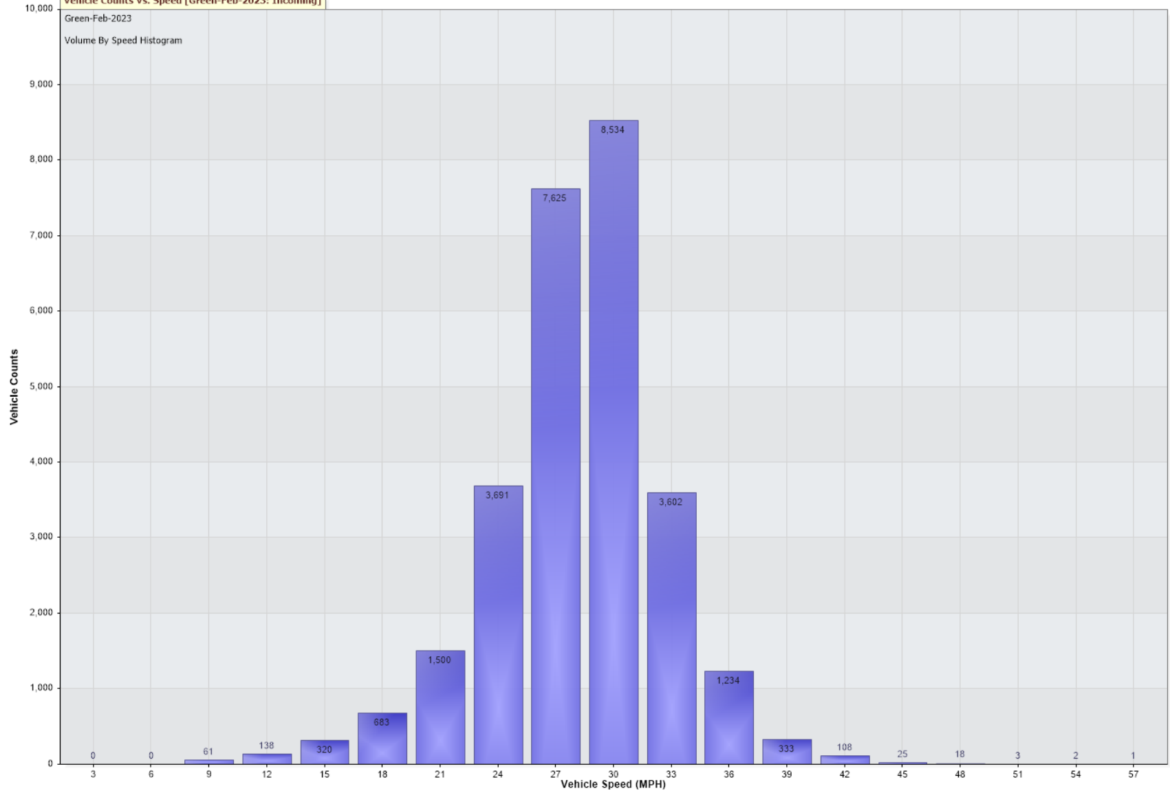
Vehicle Counts Vs. Speed [Green-Feb-2023: Incoming]
