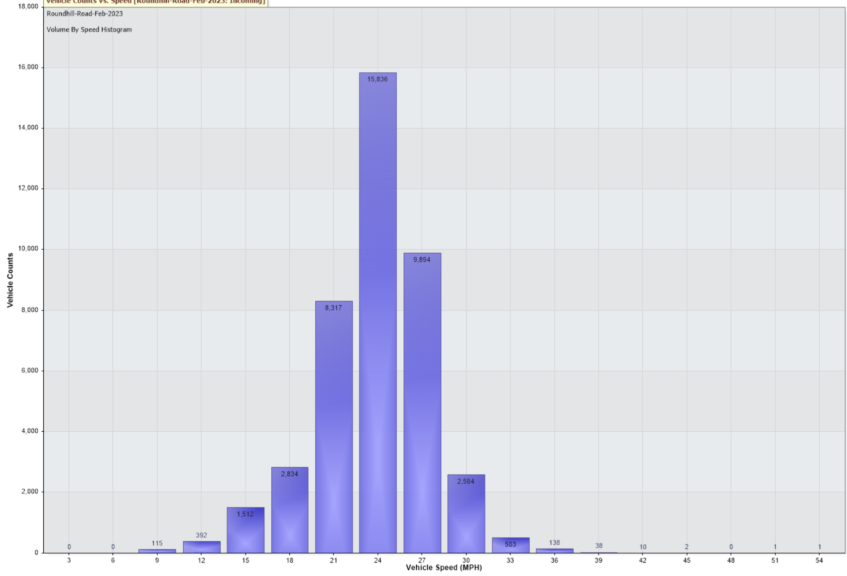
Vehicle Counts Vs. Speed [Roundhill-Road-Feb-2023: Incoming]
