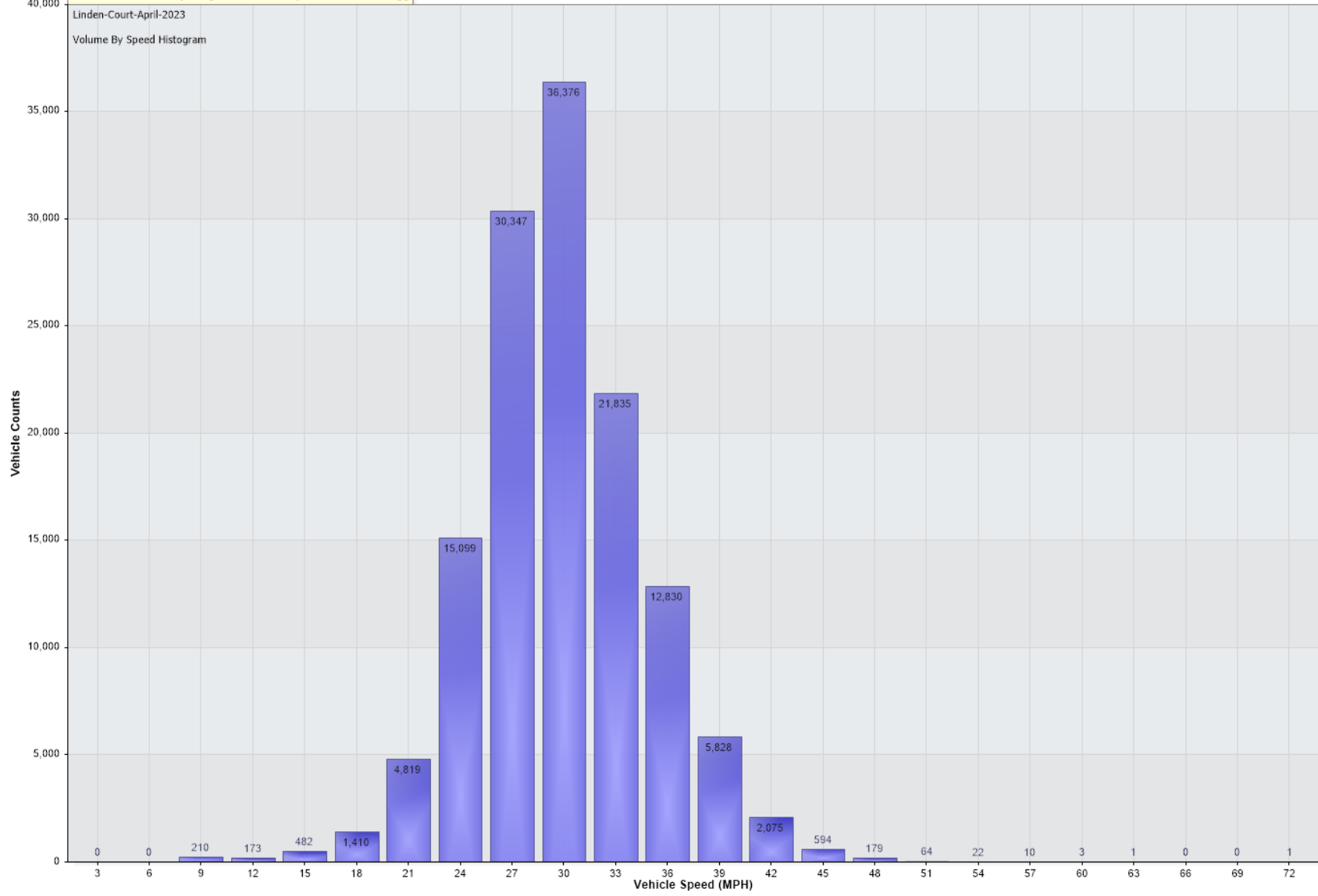
Vehicle Counts Vs. Speed [Linden-Court-April-2023: Incoming]
