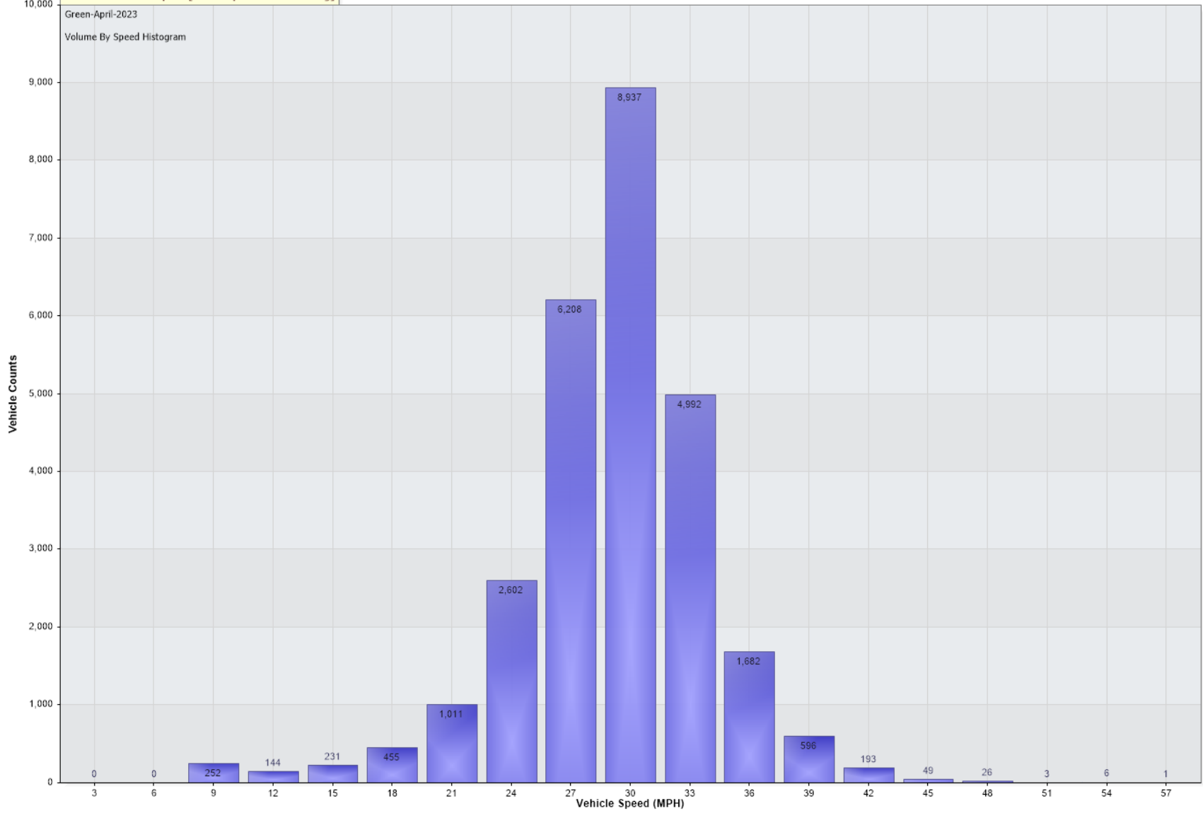
Vehicle Counts Vs. Speed [Green-April-2023: Incoming]
