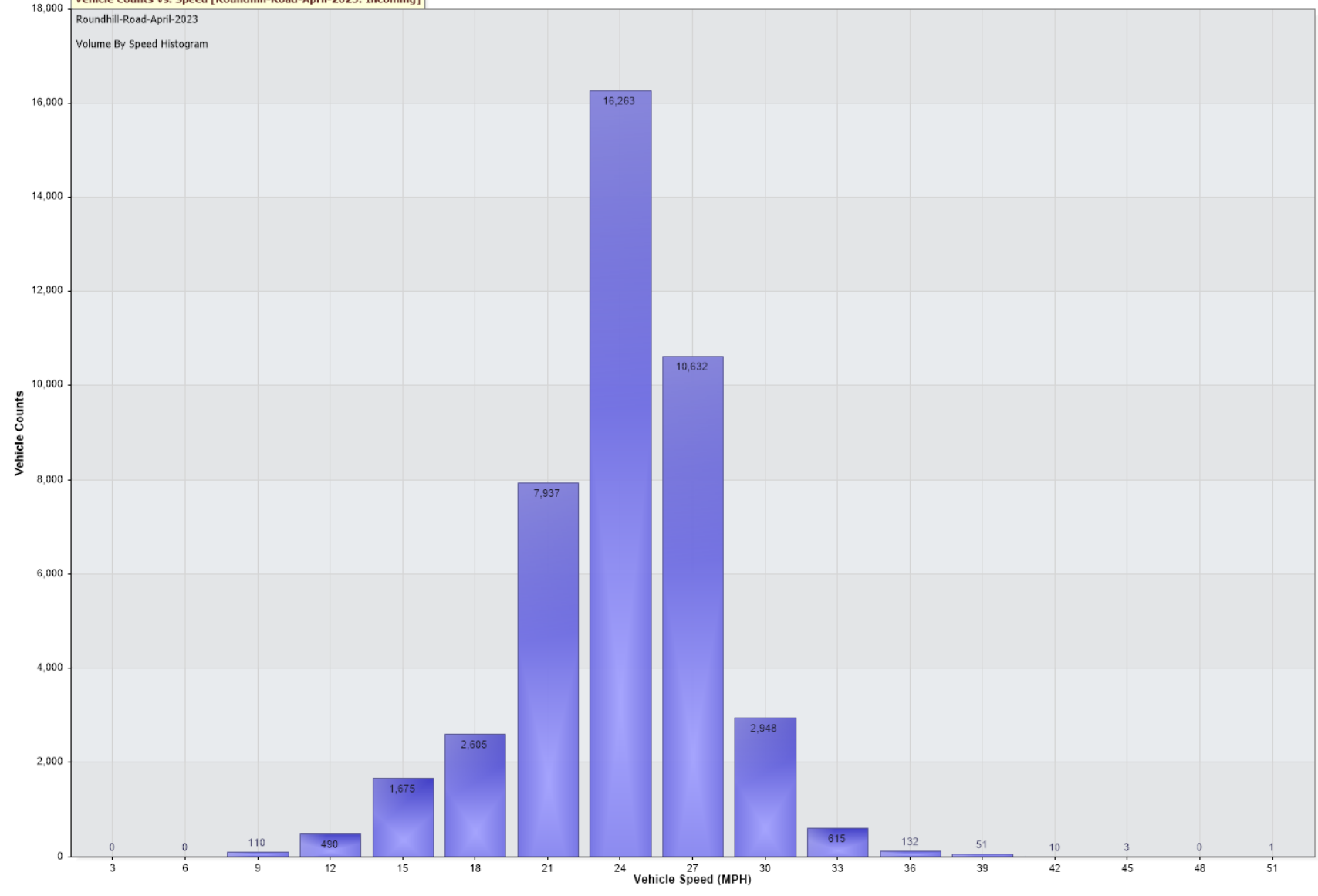
Vehicle Counts Vs. Speed [Roundhill-Road-April-2023: Incoming]
