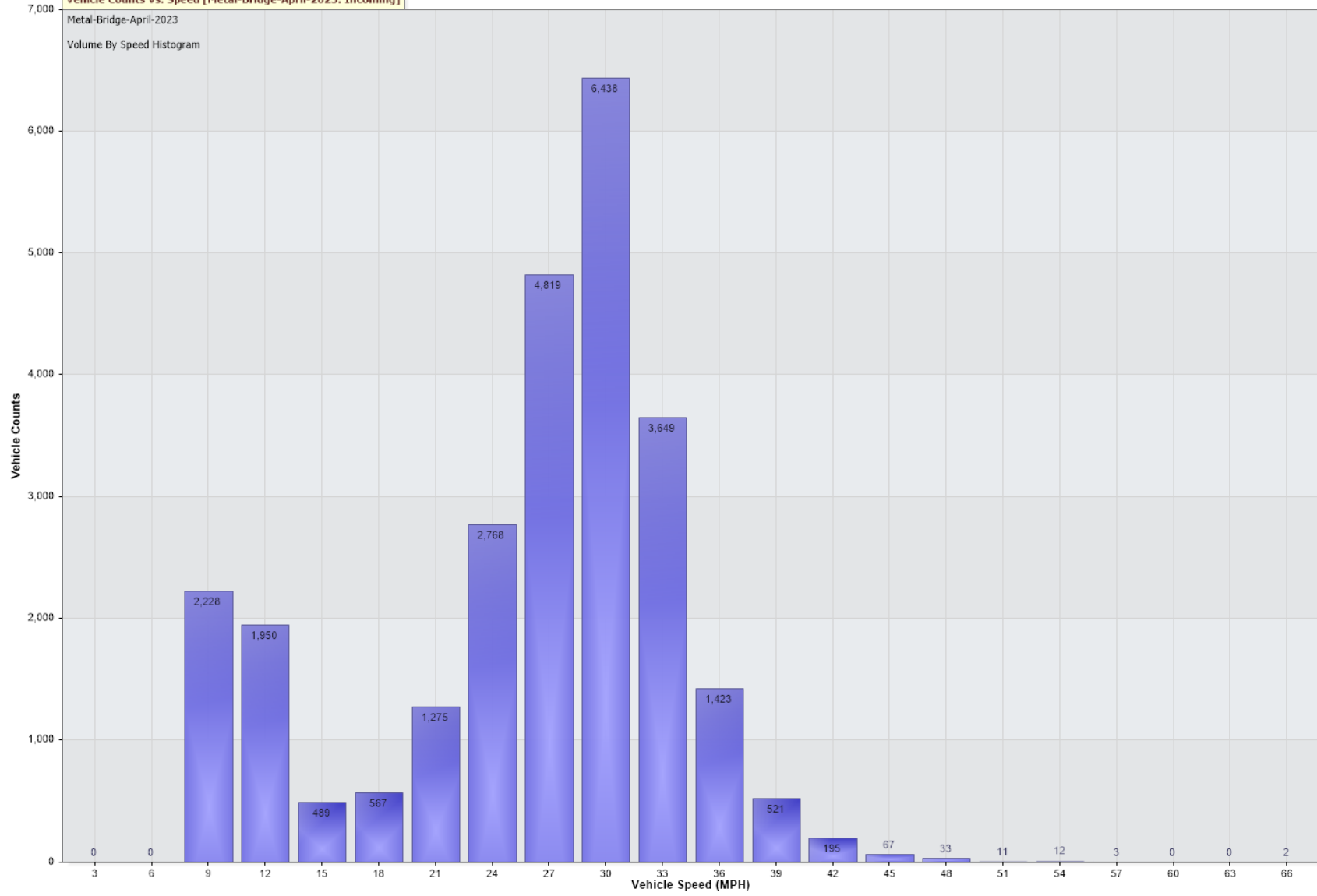
Vehicle Counts Vs. Speed [Metal-Bridge-April-2023: Incoming]
