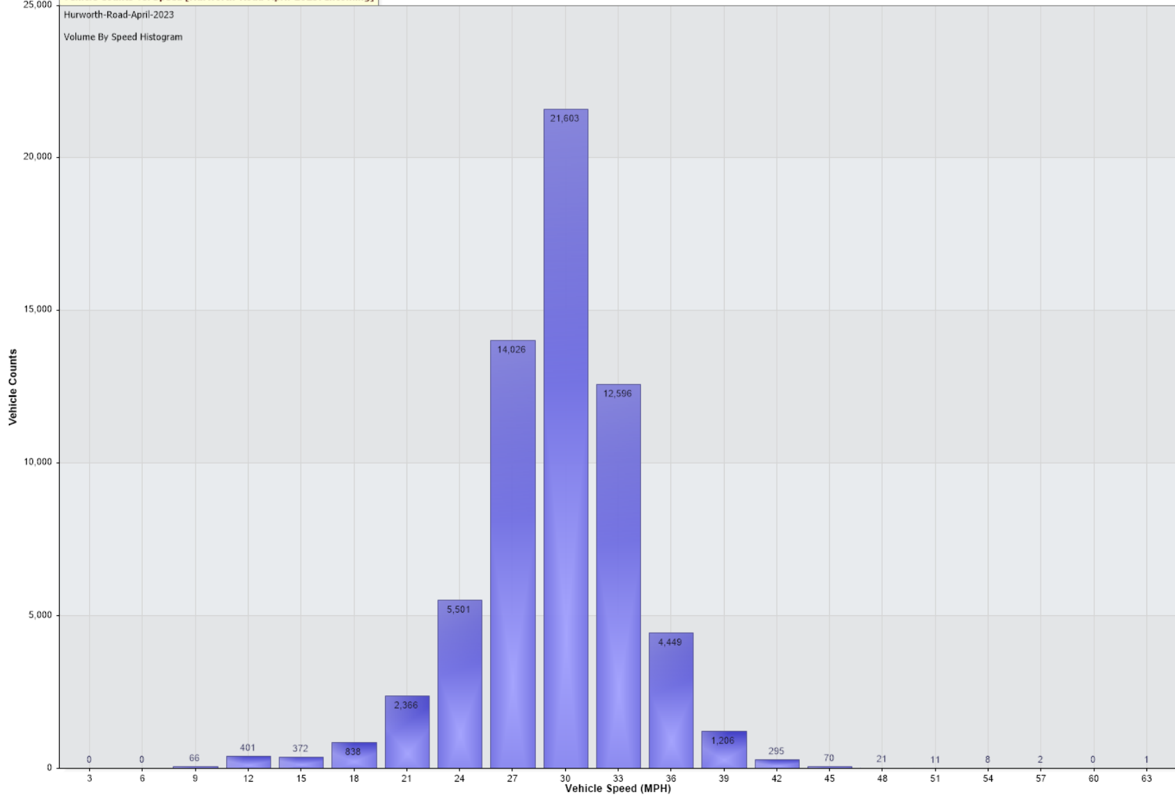
Vehicle Counts Vs. Speed [Hurworth-Road-April-2023: Incoming]
